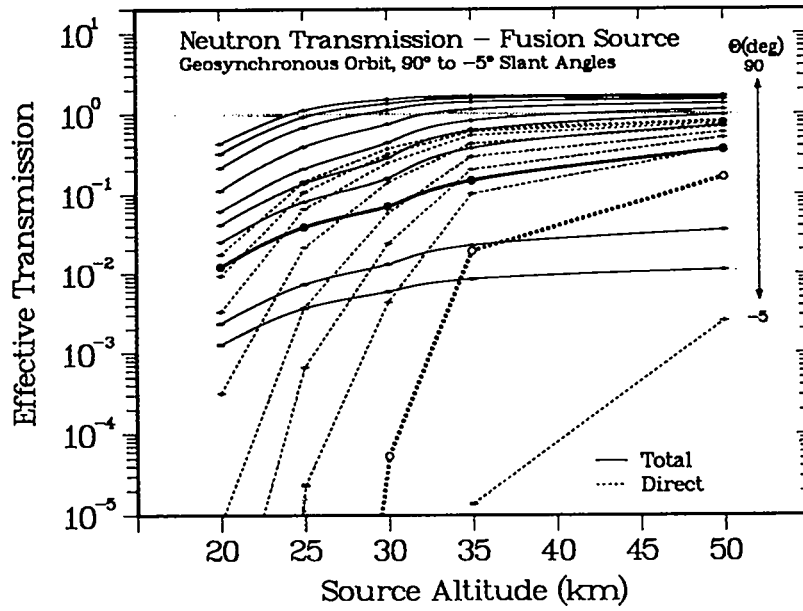
Fig. 3.2a. As in Fig. 3.1a, but for the altitude dependence of the integrated fusion fluences at different slant angles.
