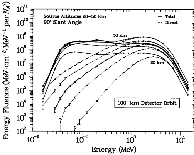
Fig. 2.6a. Energy-weighted photon fluences from sources with altitudes varying from 20 km to 50 km. The detector is in a 100-km orbit and is directly above the source.
