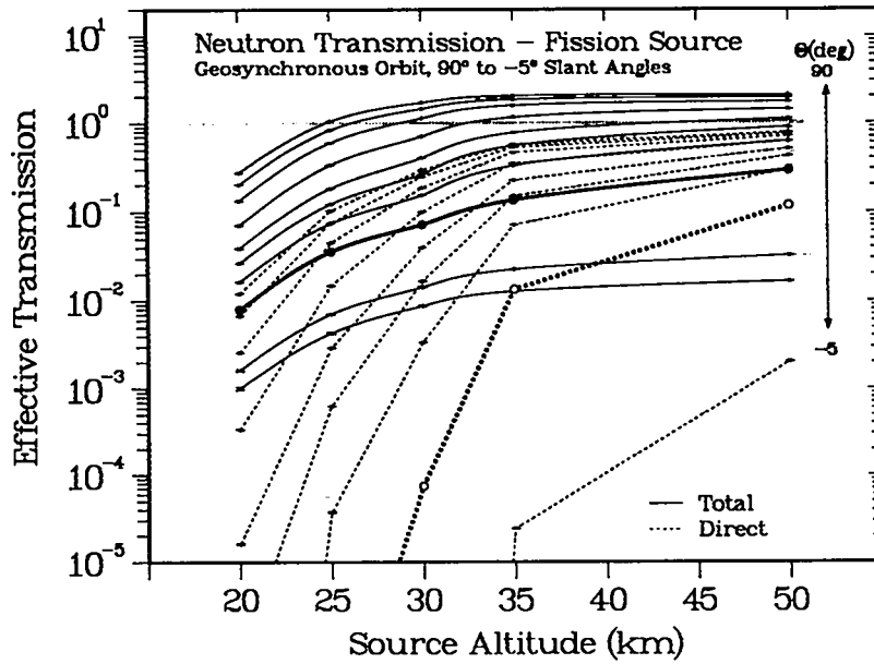
Fig. 3.2b. Transmissions as in Fig. 3.1b, but for altitude dependence.
