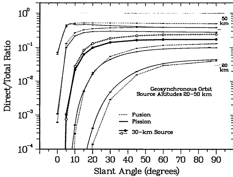
Fig. 3.3a. Direct-to-total ratios for fission and fusion sources as a function of slant angle.
