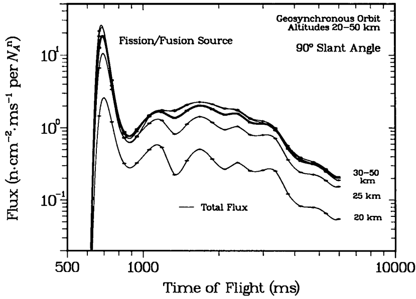
Fig. 3.11a. Neutron time-of-flight spectra from fission/fusion sources at 20-50 km as observed in a geosynchronous orbit using an extreme slant angle of 90^\circ .
