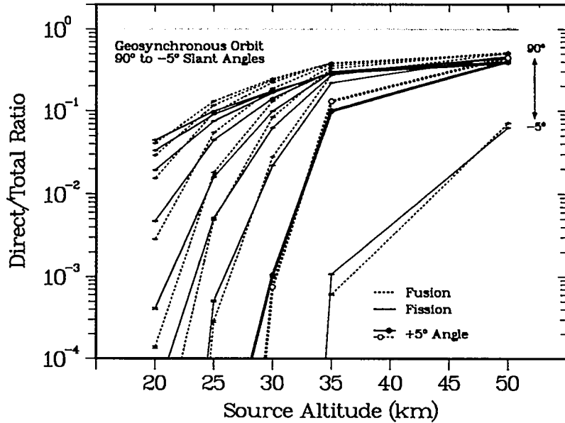
Fig. 3.3b. Direct-to-total ratios for fission and fusion sources as a function of source altitude.
