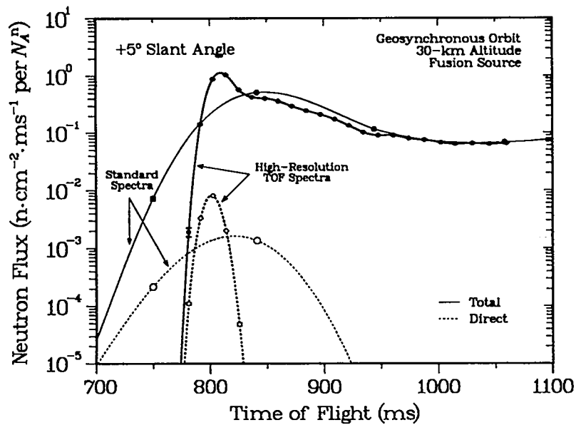
Fig. 3.7b. Detailed calculation of the time-of-flight spectrum for a 30-km source altitude and +5° slant angle, emphasizing the importance of fine time steps at high energies.
