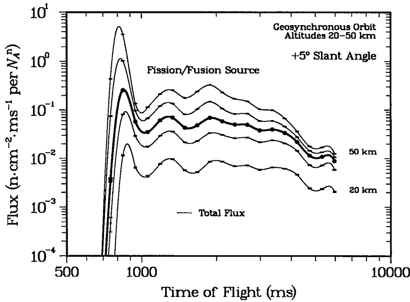
Fig. 3.11b. Neutron time-of-flight spectra as in Fig. 3.11a, but for a slant angle of +5^\circ .
