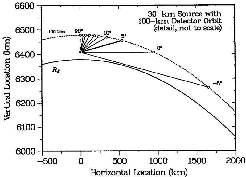
Fig. 1.1c. Geometry for the calculations, expanded vertically (that is, not to scale) to show the nearness to the Earth's surface for the paths at the two lowest slant angles.
